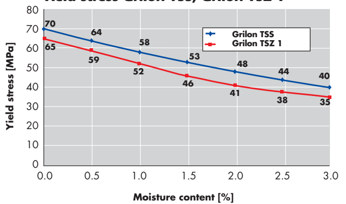
Yield stress Grilon TSS, Grilon TSZ 1
