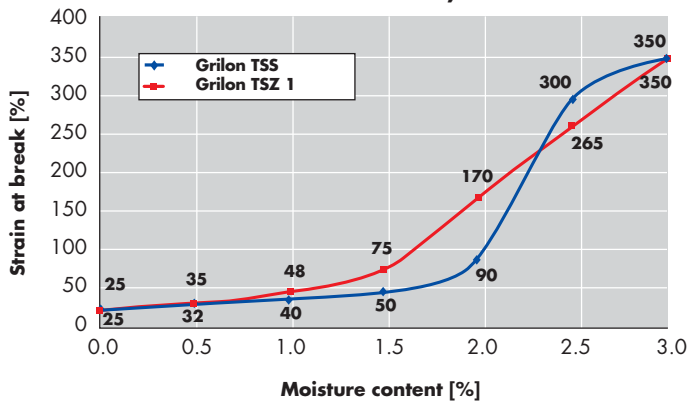
Strain at break Grilon TSS, Grilon TSZ 1
