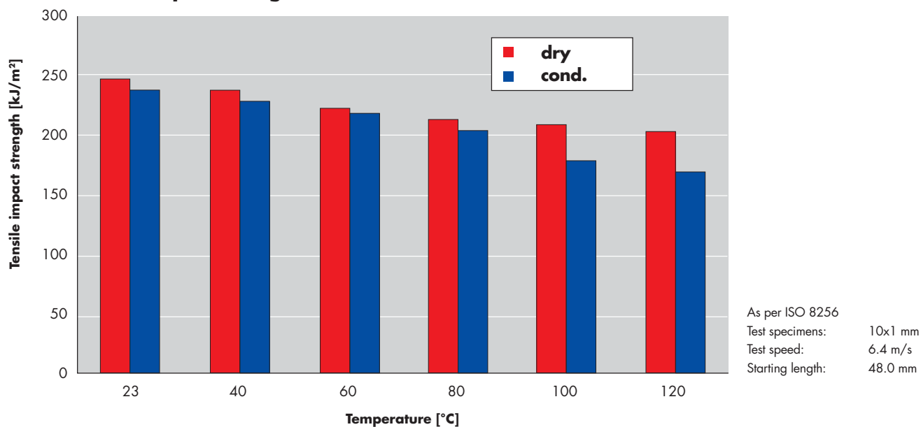
Tensile impact strength Grilon BGZ-50/2
